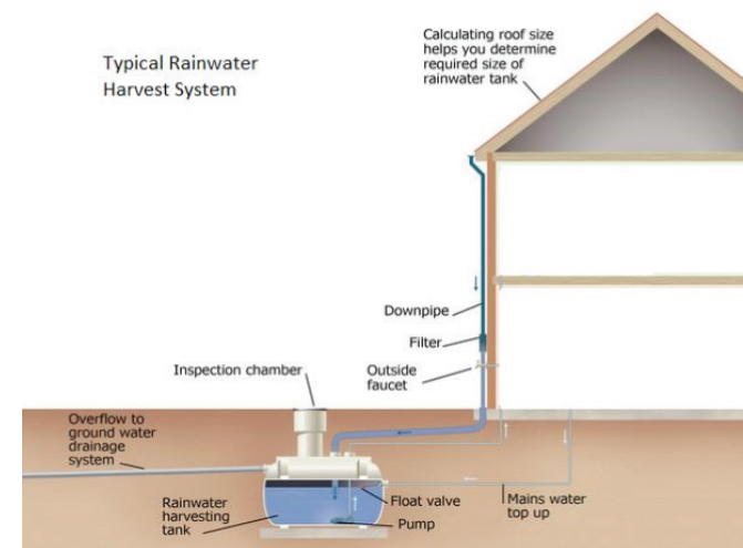
Typical Rainwater Harvest System
